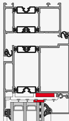
RC2 - special glass additional shimming + gluing
