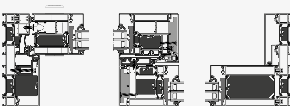
③ Lift & slide sash
