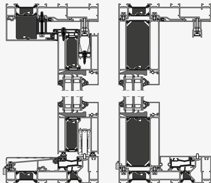
① Lift and slide sash (FO)
