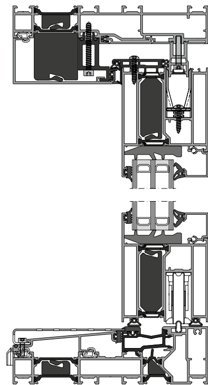
1 Lift-and-slide sash (PO)
