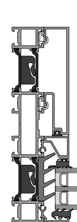
3 Direct glazing
