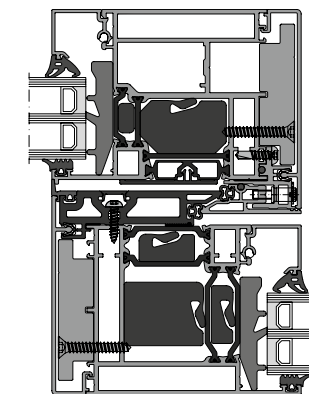
4 Mullion joint
