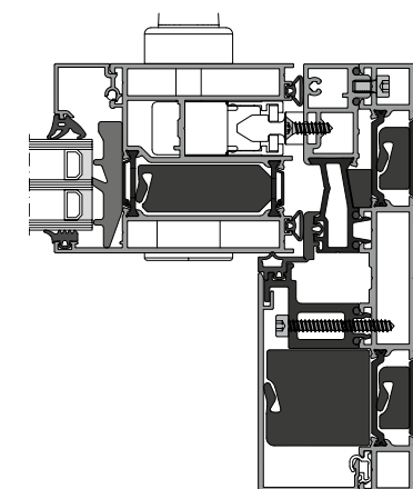
6 Lift-and-slide sash
