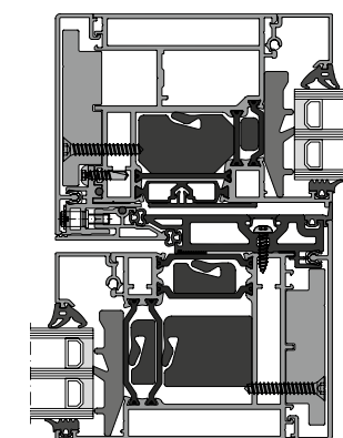
5 Mullion joint
