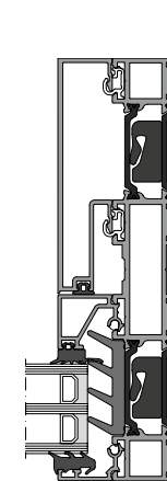
6 Direct glazing
