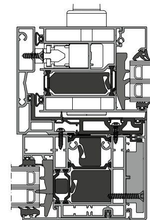
4 Mullion joint
