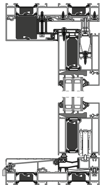
1 Lift-and-slide sash
