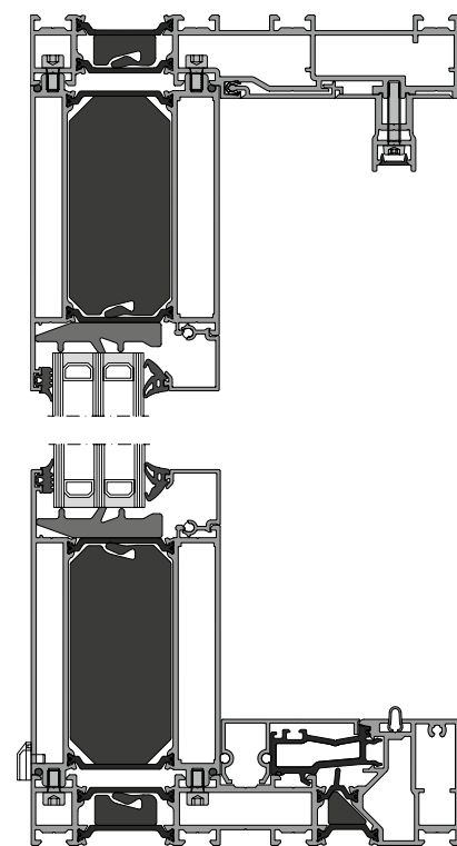
2 Fixed glazing profile (PO)
