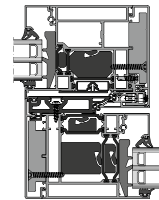
6 Mullion joint
