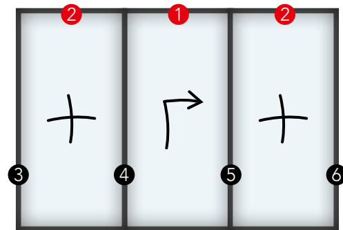
System configuration G+: 1 lift-and-slide sash + 2 fixed glazed panels
