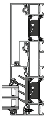
7 Direct glazing
