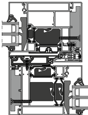
4 Mullion joint
