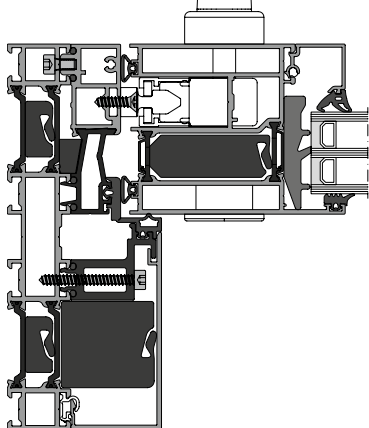
3 Lift-and-slide sash
