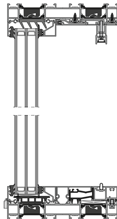
2 Direct glazing
