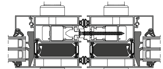
5 Dummy mullion
