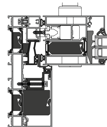
3 Lift-and-slide sash
