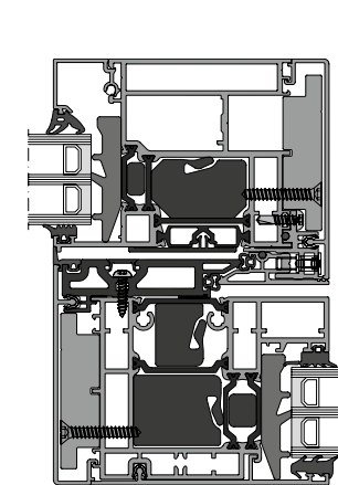
5 Mullion joint
