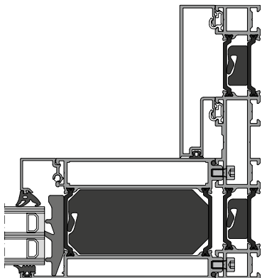
5 Fixed glazing profile
