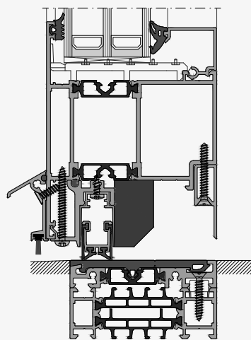
Outward opening Barrier-free zero threshold
