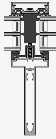
THERM + 50 A-V with insulating block P and T structural profile
